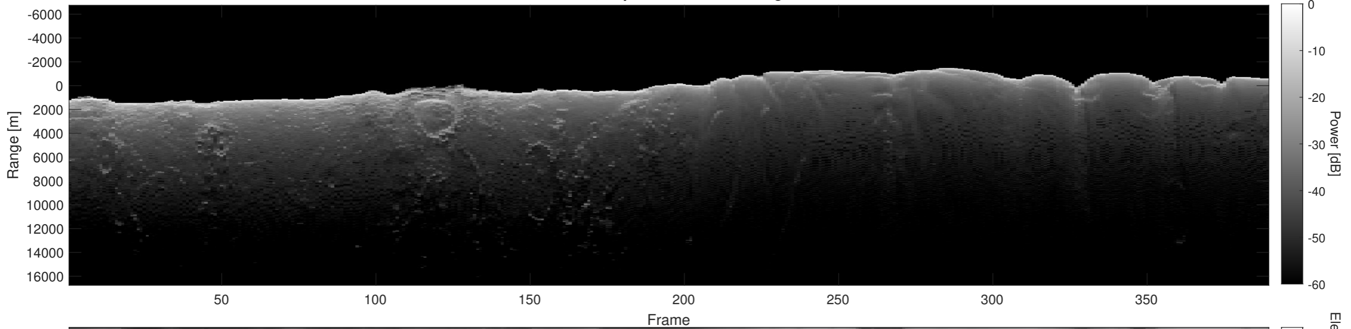
Orbit 4425, Depth-Corrected Cluttergram
