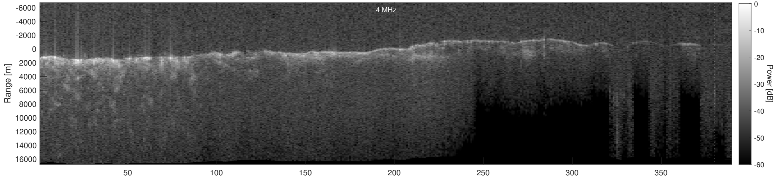
Orbit 4425, Depth-Corrected Cluttergram
