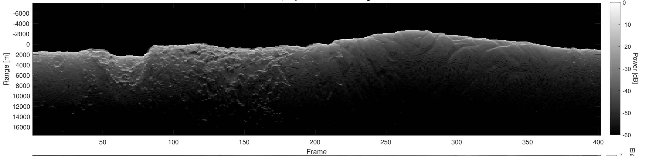
Orbit 4426, Depth-Corrected Cluttergram
