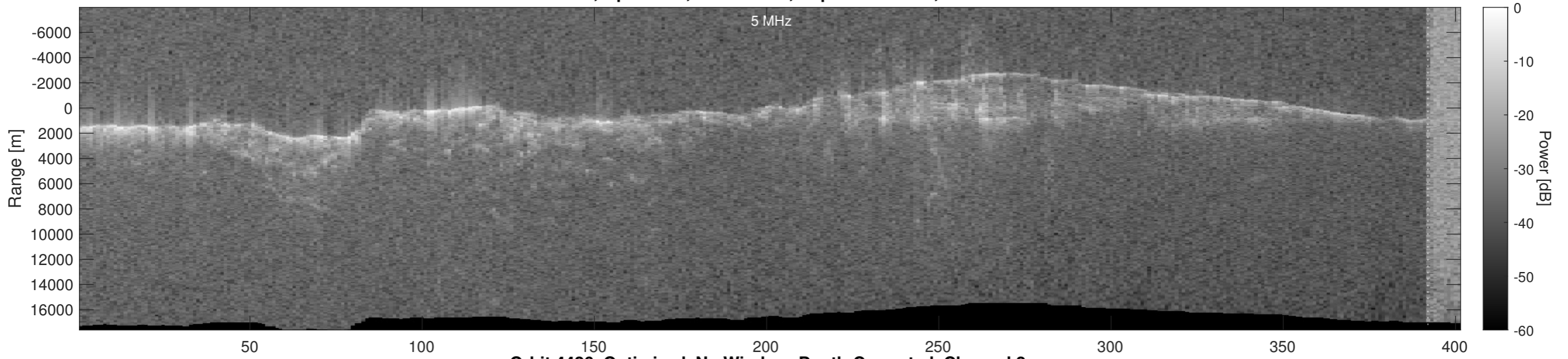
Orbit 4426, Optimized, No Window, Depth-Corrected, Channel 2
