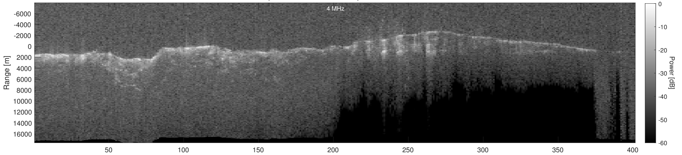
Orbit 4426, Depth-Corrected Cluttergram
