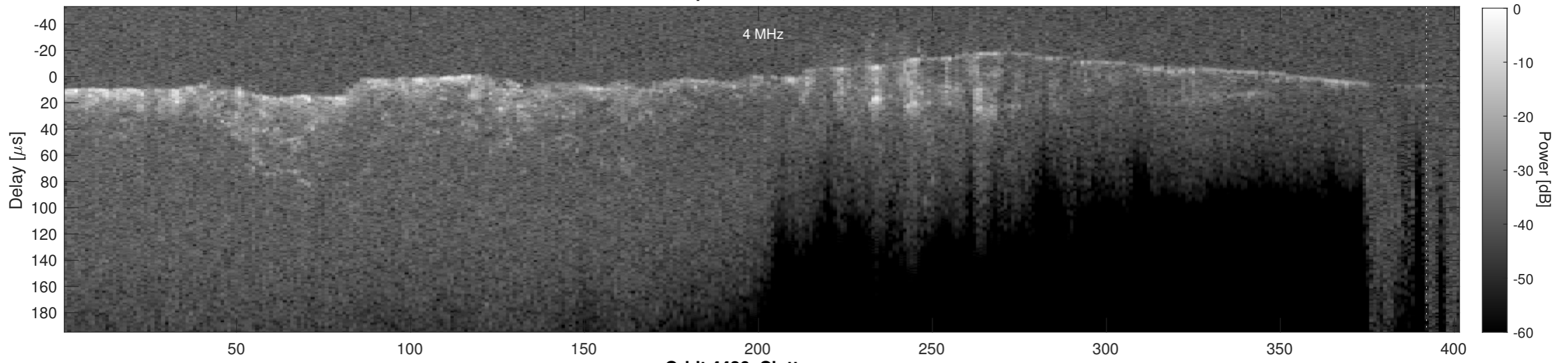
Orbit 4426, Cluttergram
