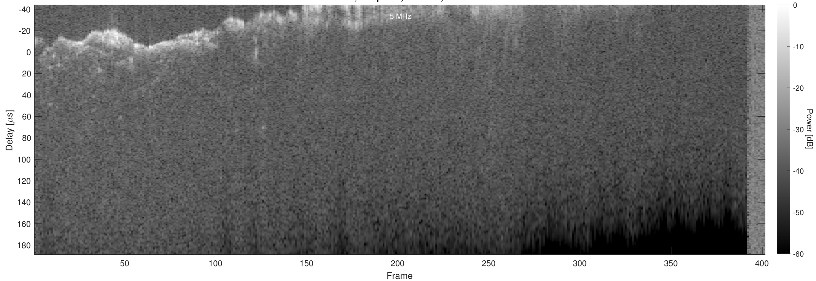
Orbit 4427, Chapman, Window, Channel 2
