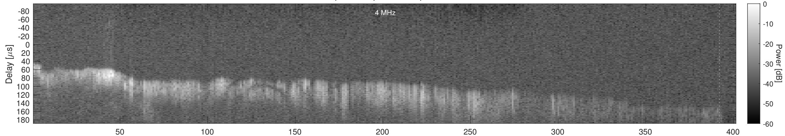
Orbit 4427, Window, Channel 2, Chapman
