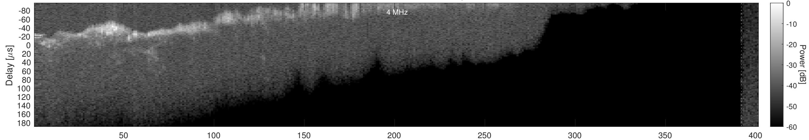
Orbit 4427, Window, Channel 2, Optimized
