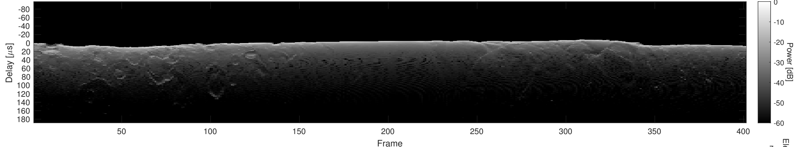
Orbit 4427, Cluttergram
