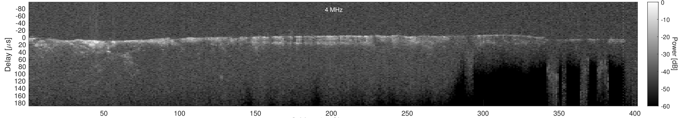
Orbit 4427, Cluttergram
