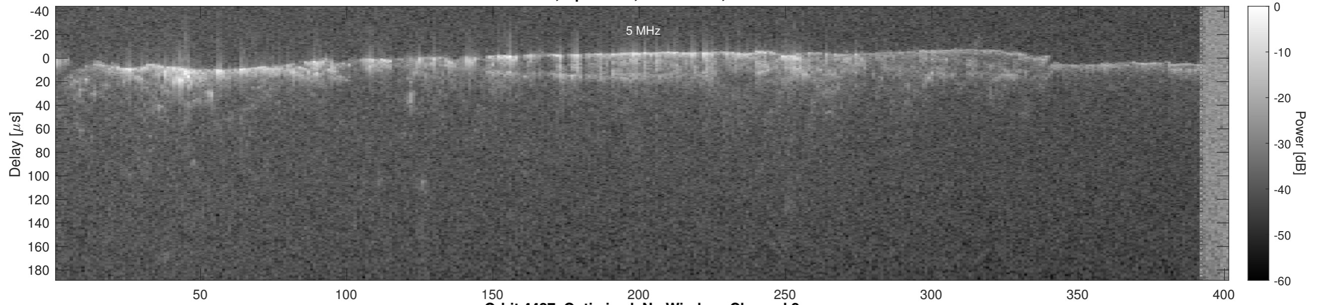
Orbit 4427, Optimized, No Window, Channel 2
