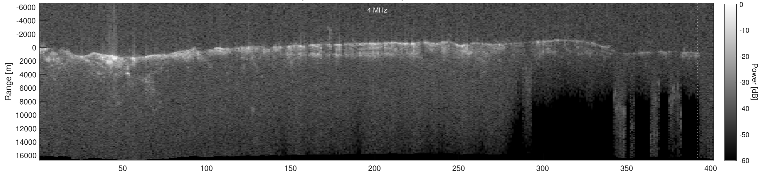
Orbit 4427, Depth-Corrected Cluttergram
