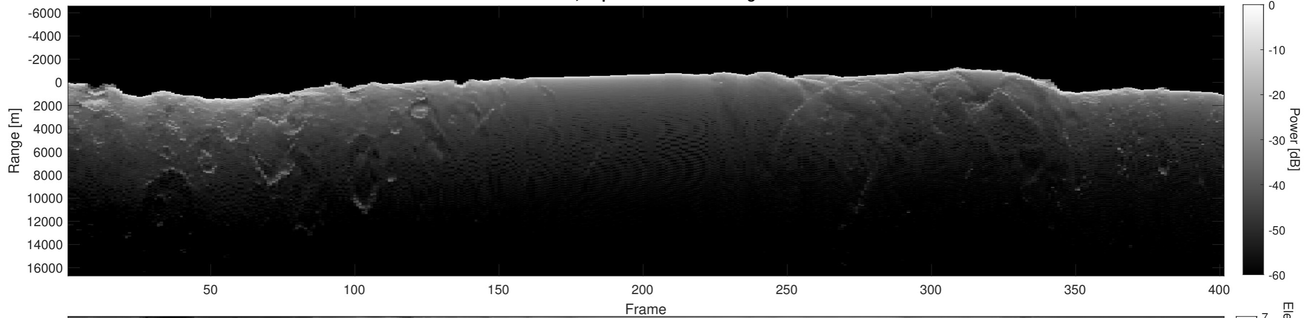
Orbit 4427, Depth-Corrected Cluttergram
