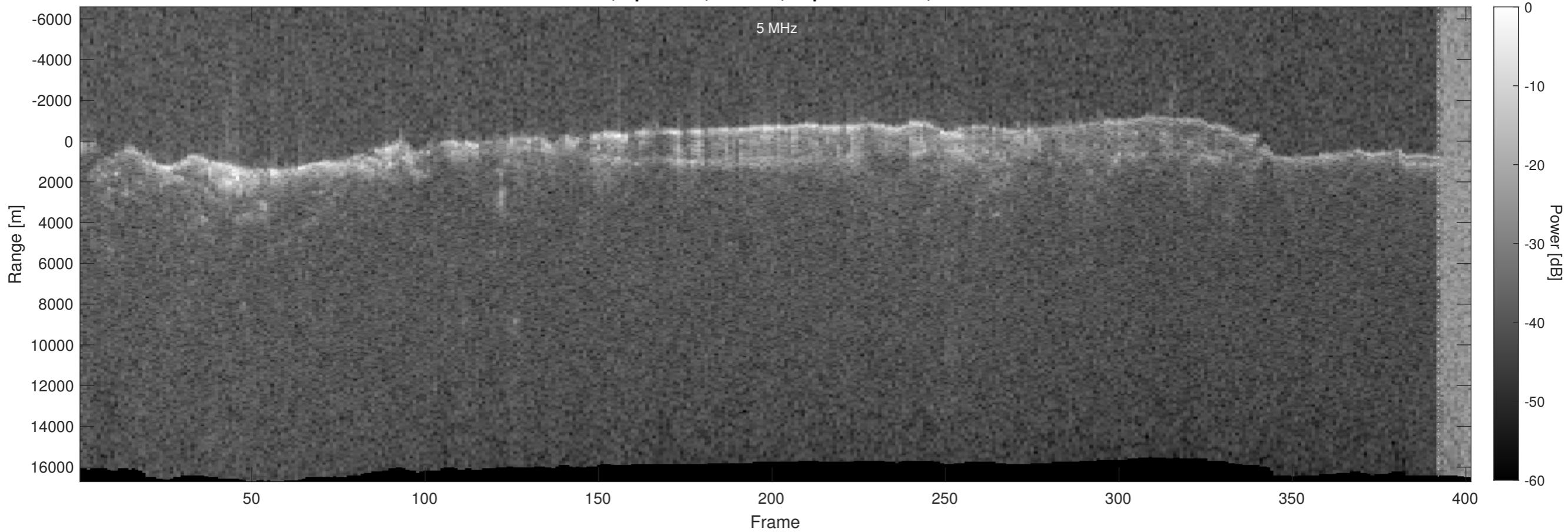
Orbit 4427, Optimized, Window, Depth-Corrected, Channel 2
