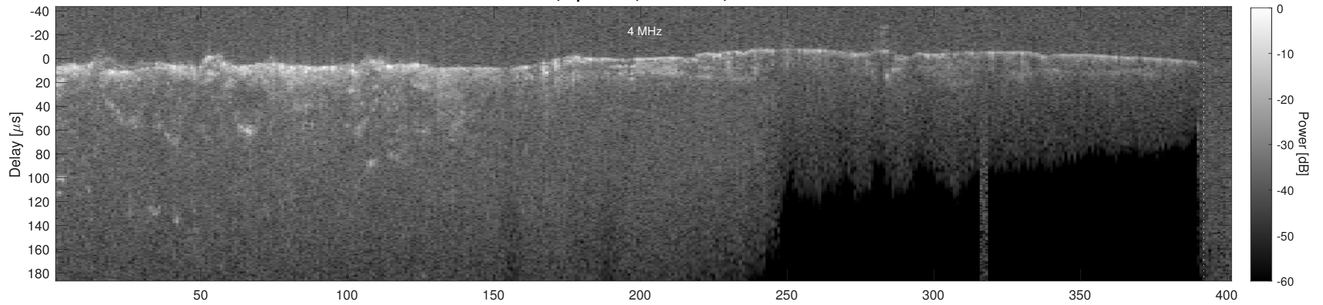
Orbit 4428, Cluttergram
