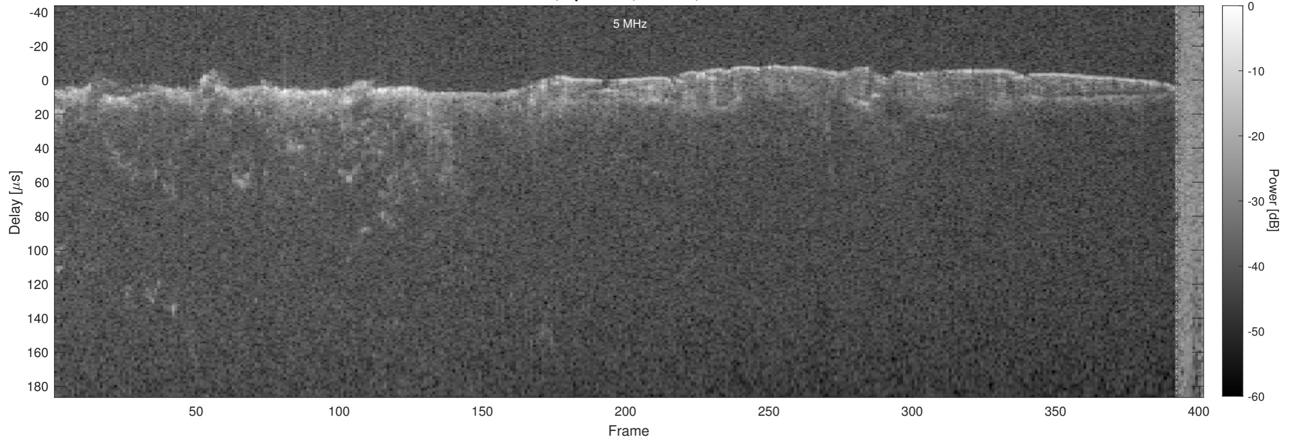
Orbit 4428, Optimized, Window, Channel 2
