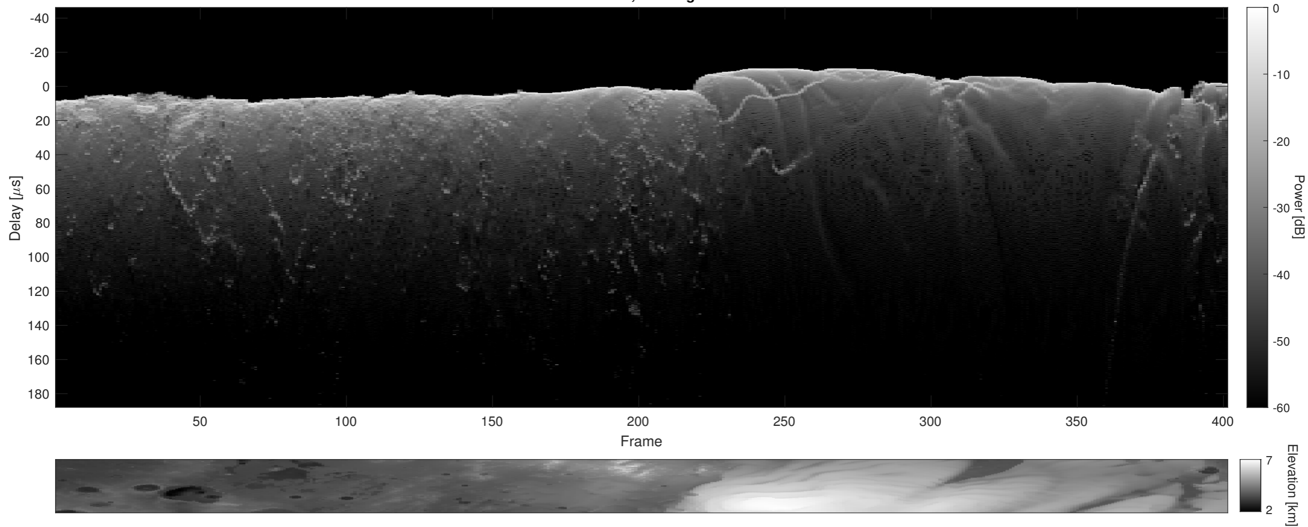
Orbit 4429, Cluttergram
