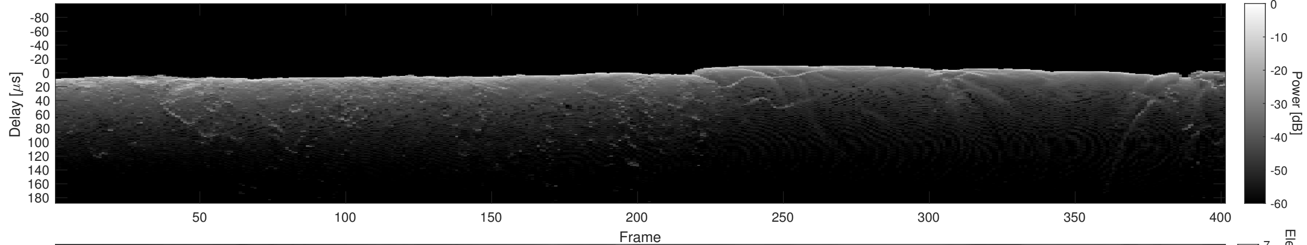
Orbit 4429, Cluttergram
