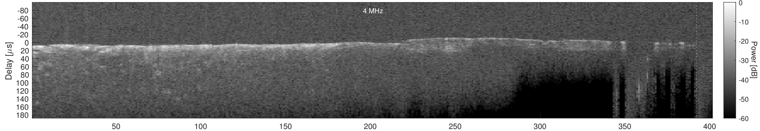
Orbit 4429, Cluttergram
