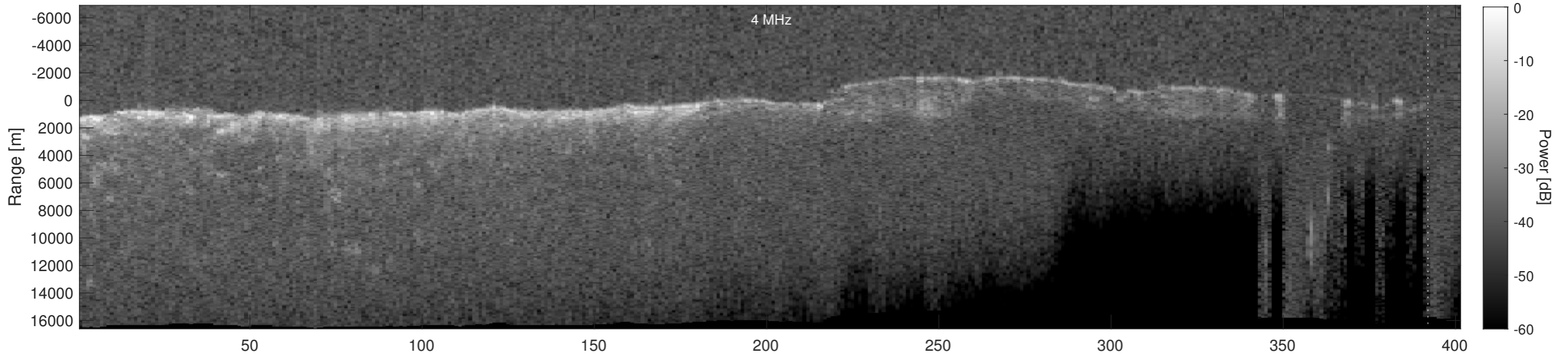
Orbit 4429, Depth-Corrected Cluttergram
