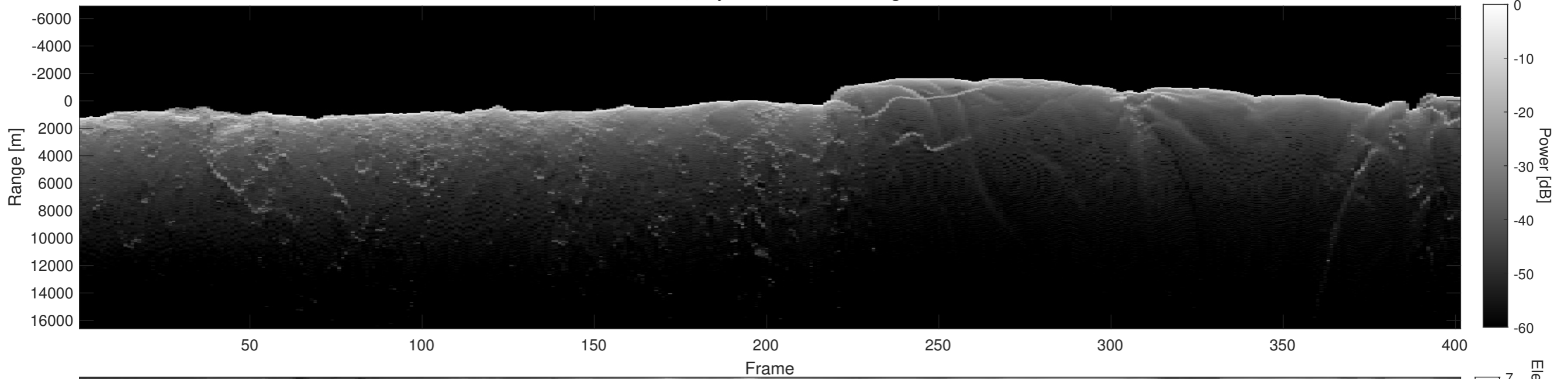
Orbit 4429, Depth-Corrected Cluttergram
