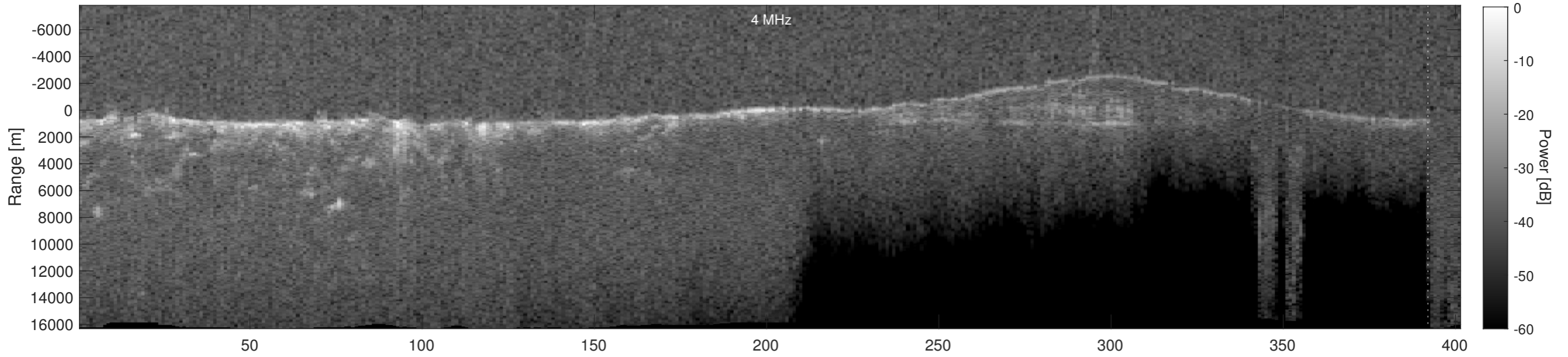
Orbit 4430, Depth-Corrected Cluttergram
