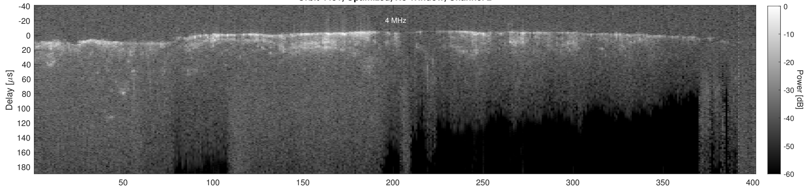
Orbit 4431, Cluttergram
