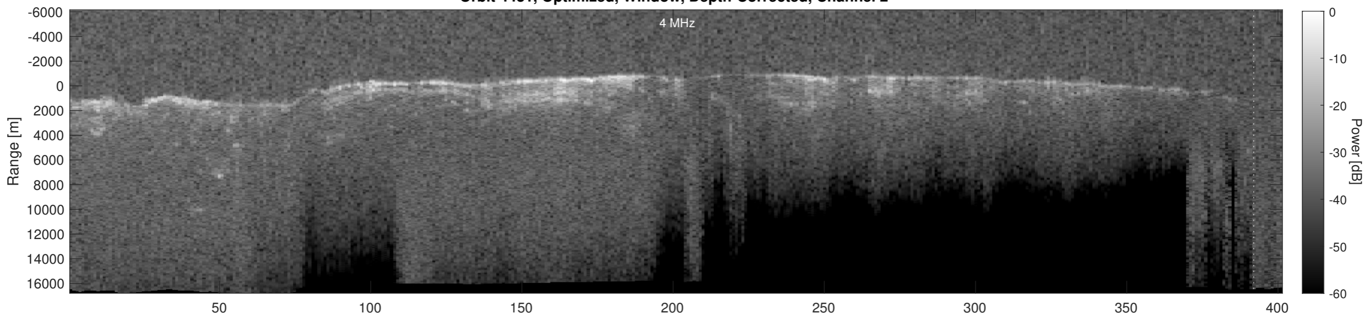
Orbit 4431, Depth-Corrected Cluttergram
