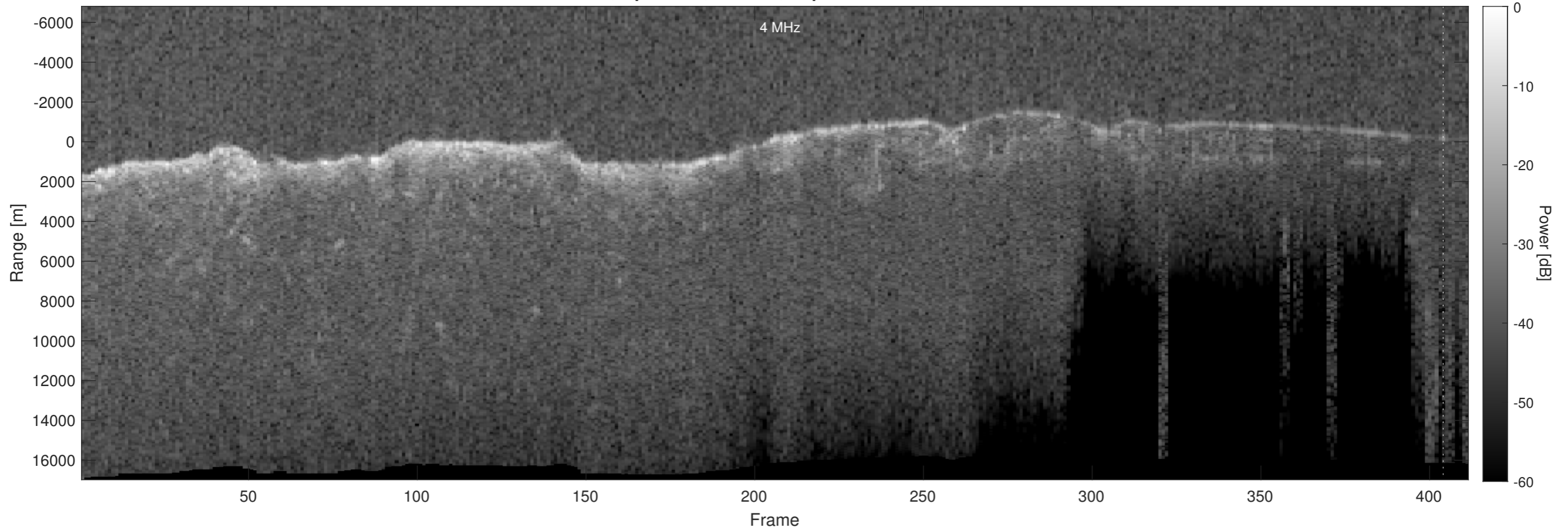
Orbit 4432, Optimized, Window, Depth-Corrected, Channel 2
