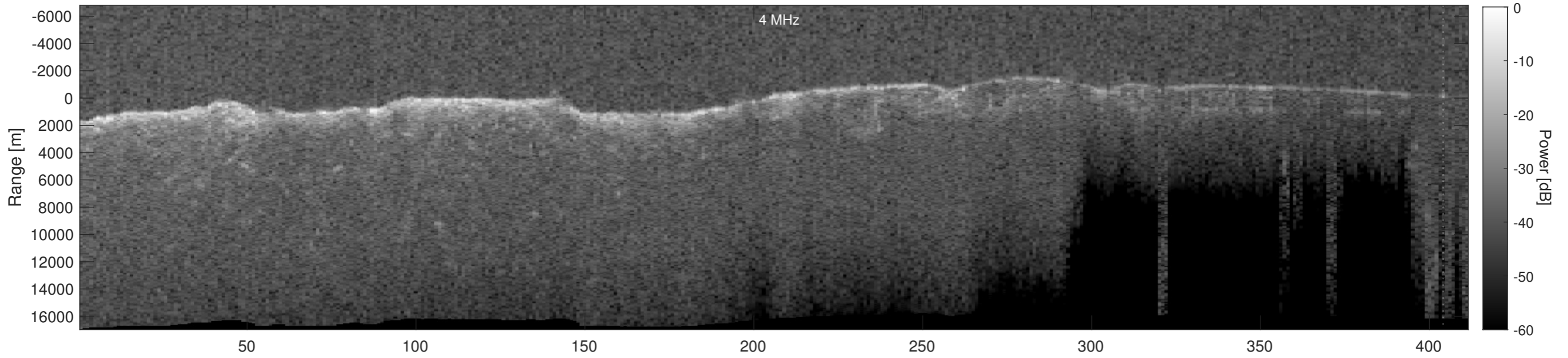
Orbit 4432, Depth-Corrected Cluttergram
