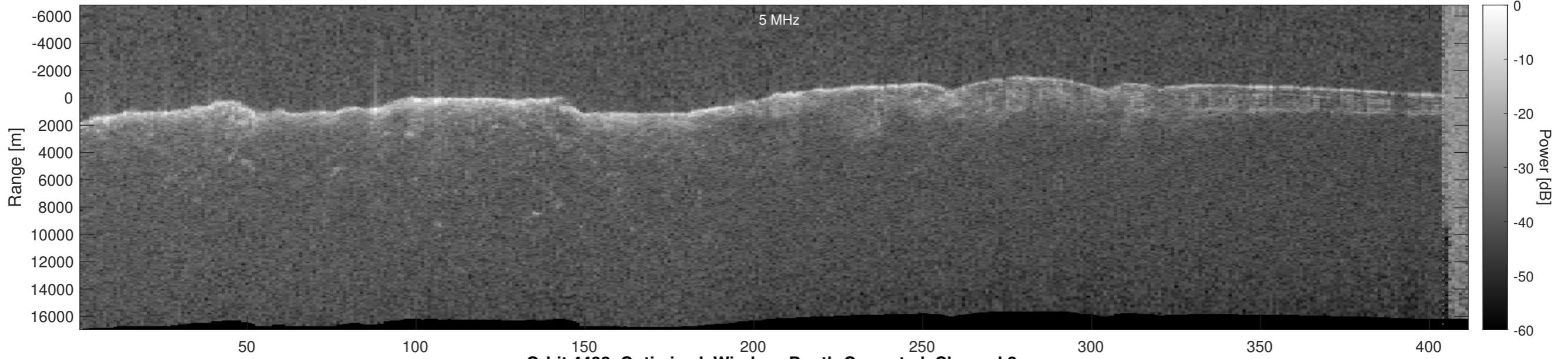
Orbit 4432, Optimized, Window, Depth-Corrected, Channel 2
