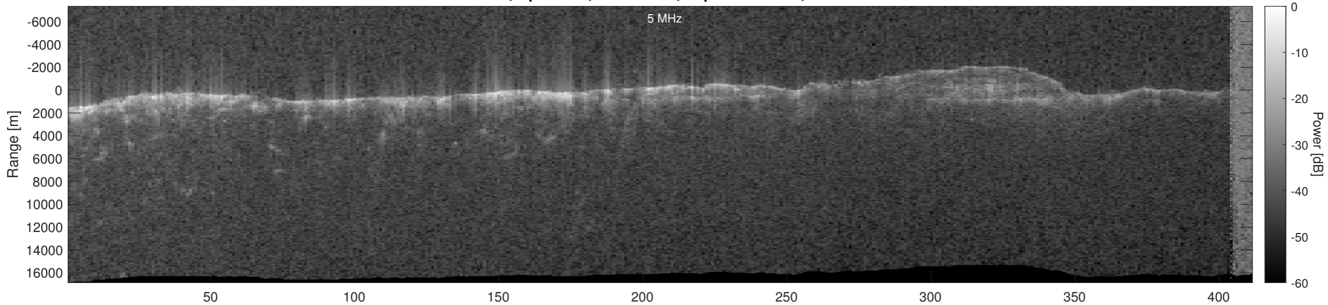
Orbit 4434, Optimized, No Window, Depth-Corrected, Channel 2
