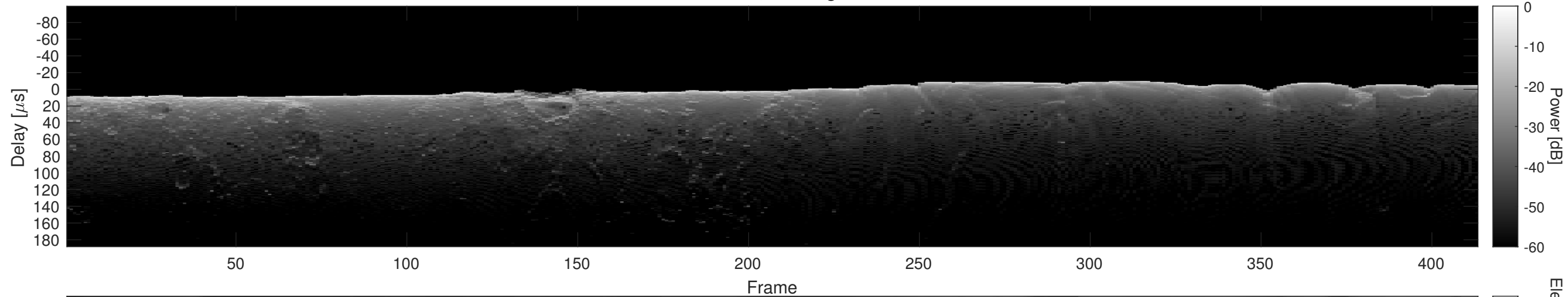
Orbit 4436, Cluttergram
