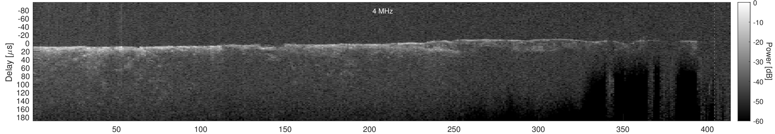
Orbit 4436, Cluttergram
