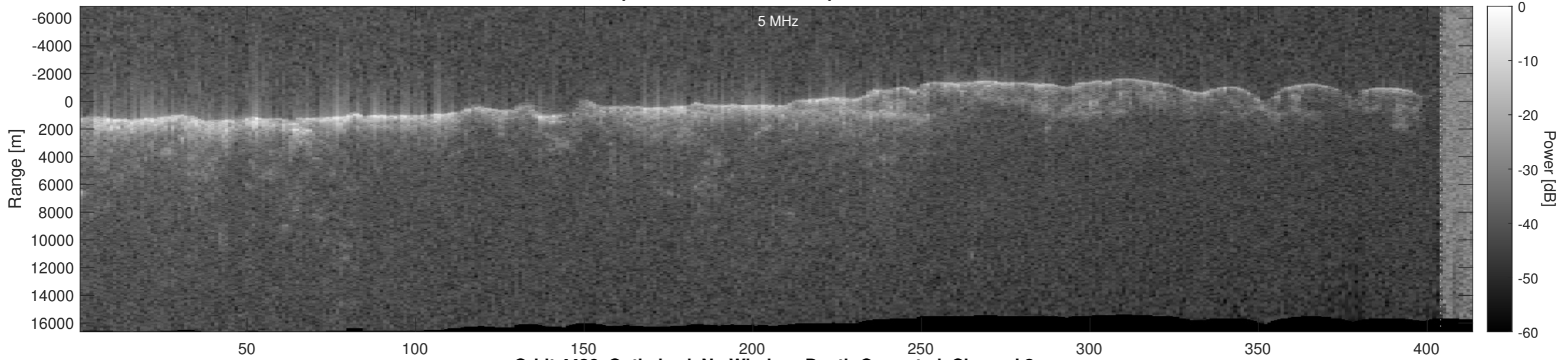
Orbit 4436, Optimized, No Window, Depth-Corrected, Channel 2
