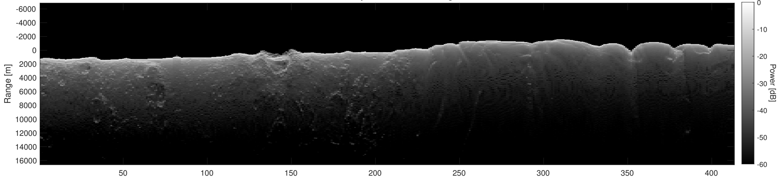
Orbit 4436, Depth-Corrected Cluttergram
