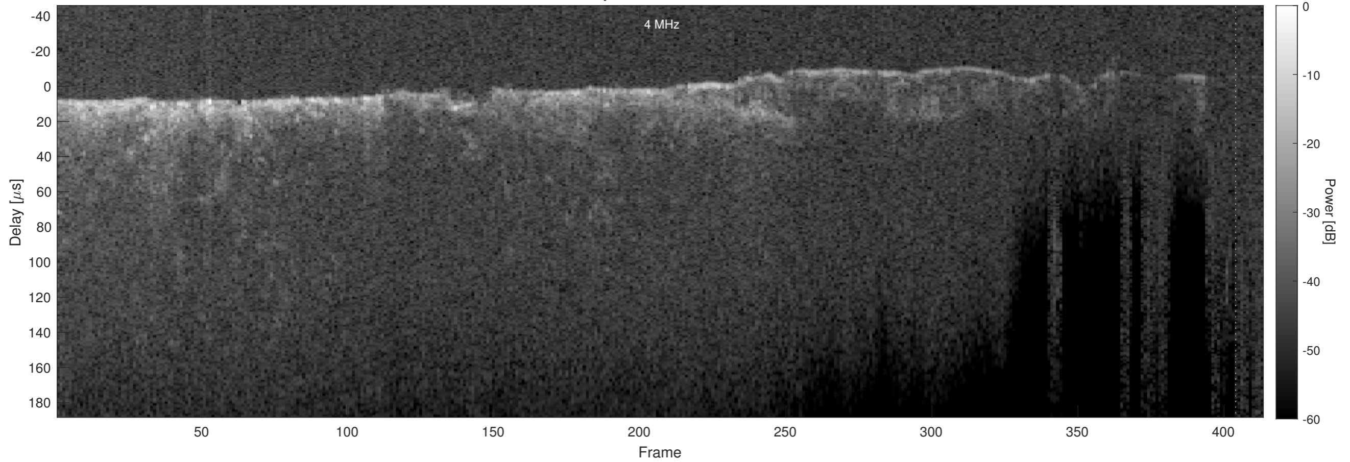
Orbit 4436, Optimized, Window, Channel 2
