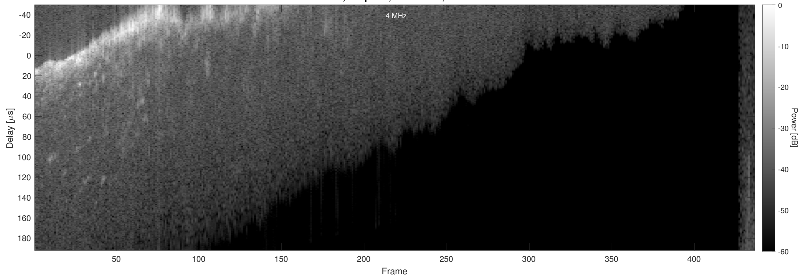
Orbit 4445, Chapman, No Window, Channel 2
