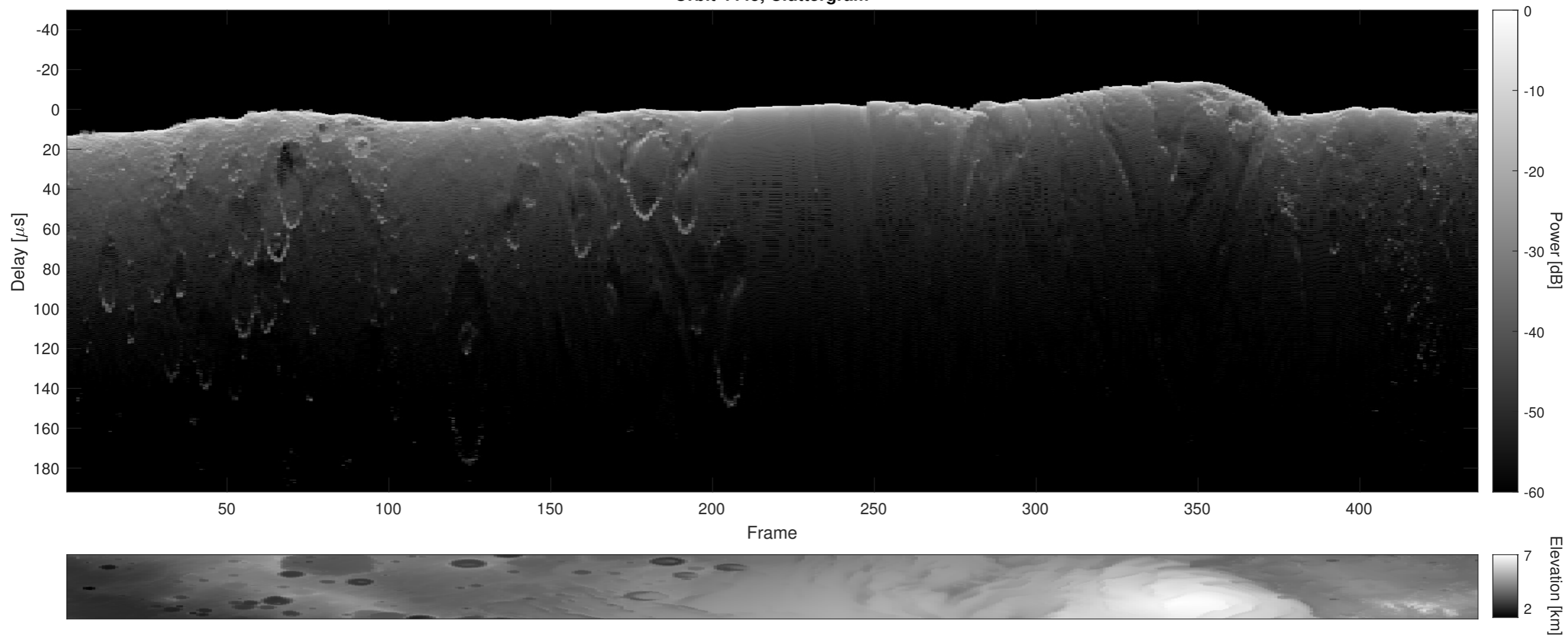
Orbit 4445, Cluttergram
