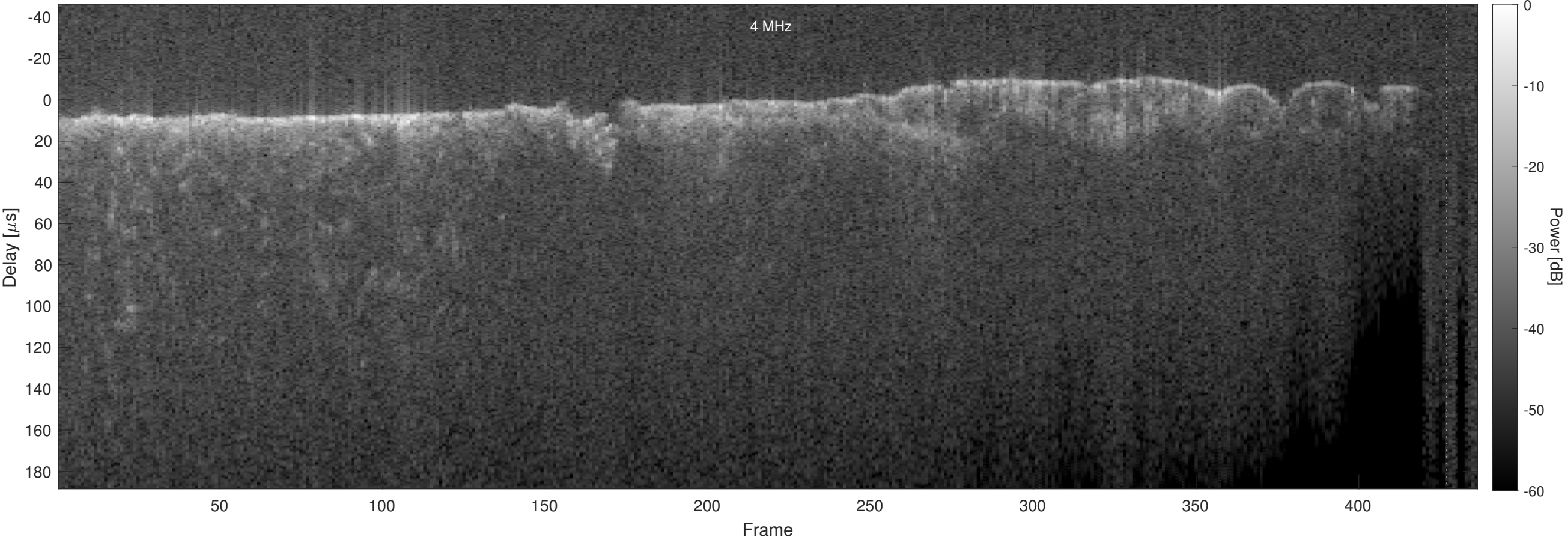
Orbit 4447, Optimized, No Window, Channel 2
