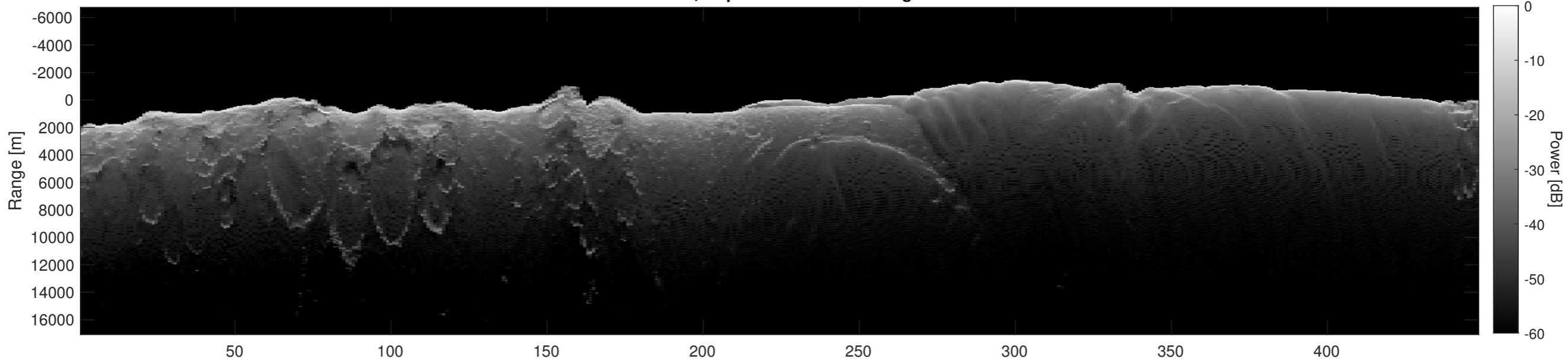
Orbit 4450, Depth-Corrected Cluttergram
