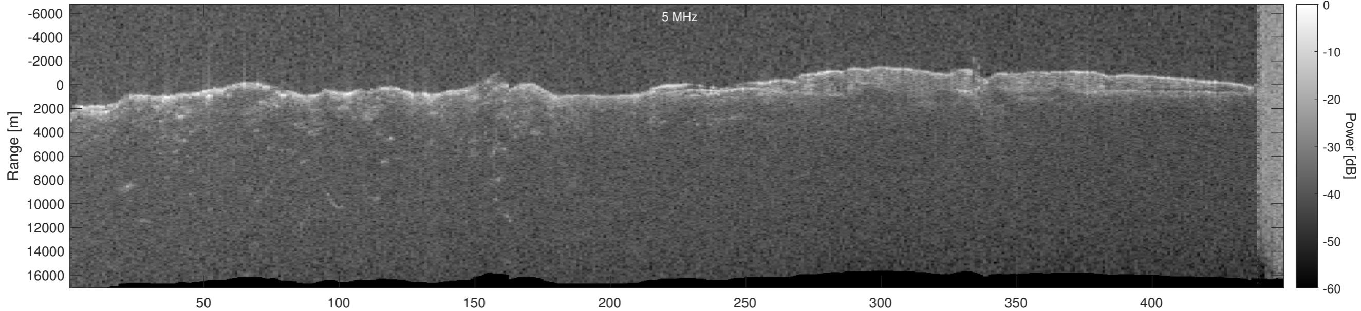
Orbit 4450, Optimized, Window, Depth-Corrected, Channel 2
