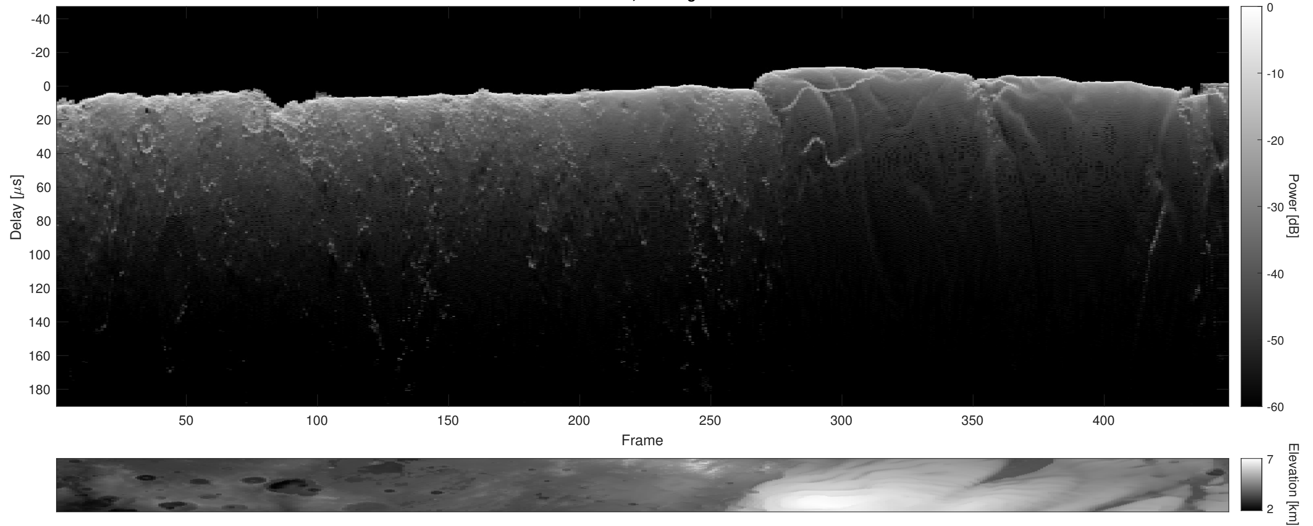
Orbit 4451, Cluttergram
