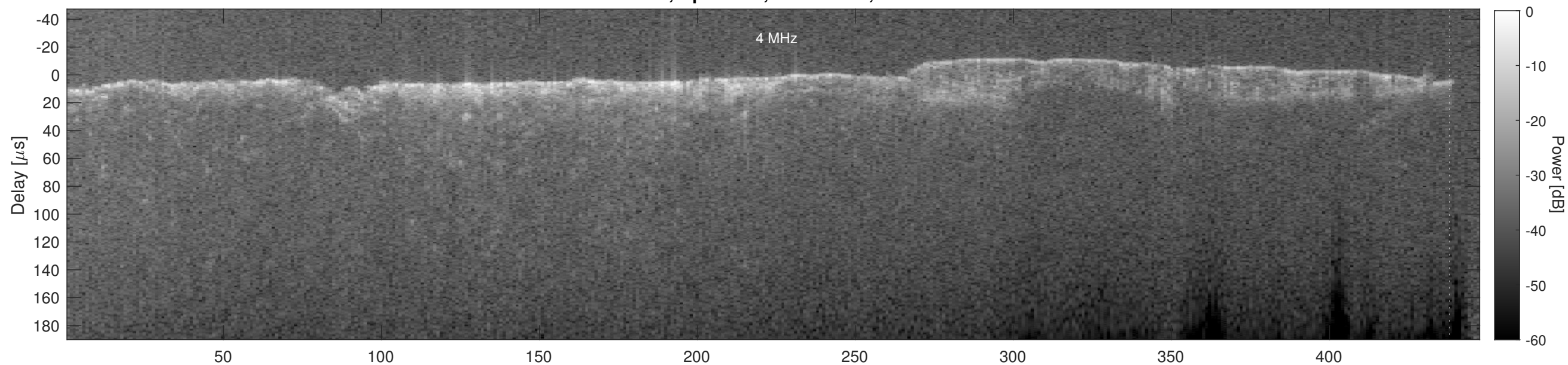
Orbit 4451, Cluttergram
