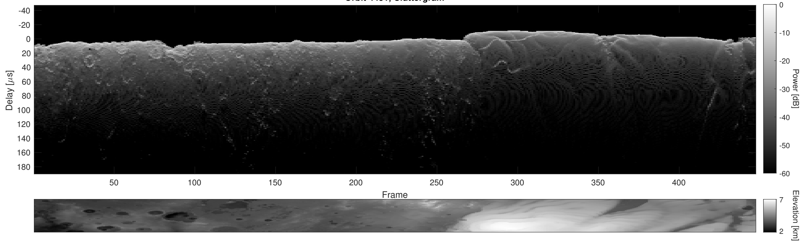
Orbit 4451, Cluttergram
