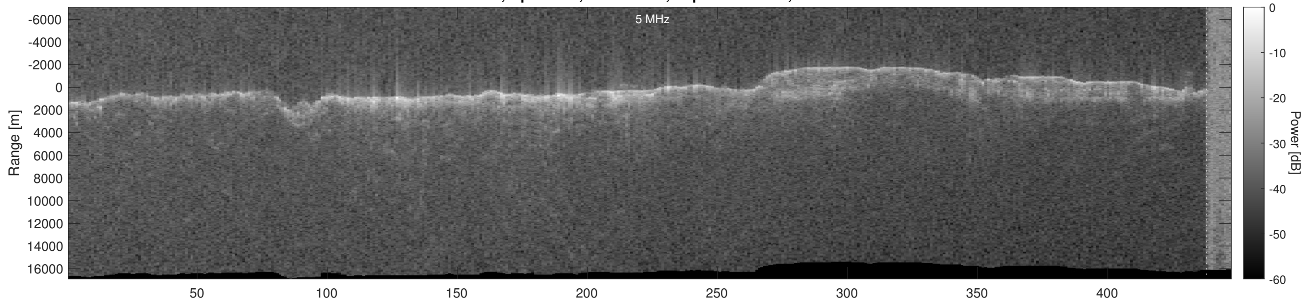
Orbit 4451, Optimized, No Window, Depth-Corrected, Channel 2
