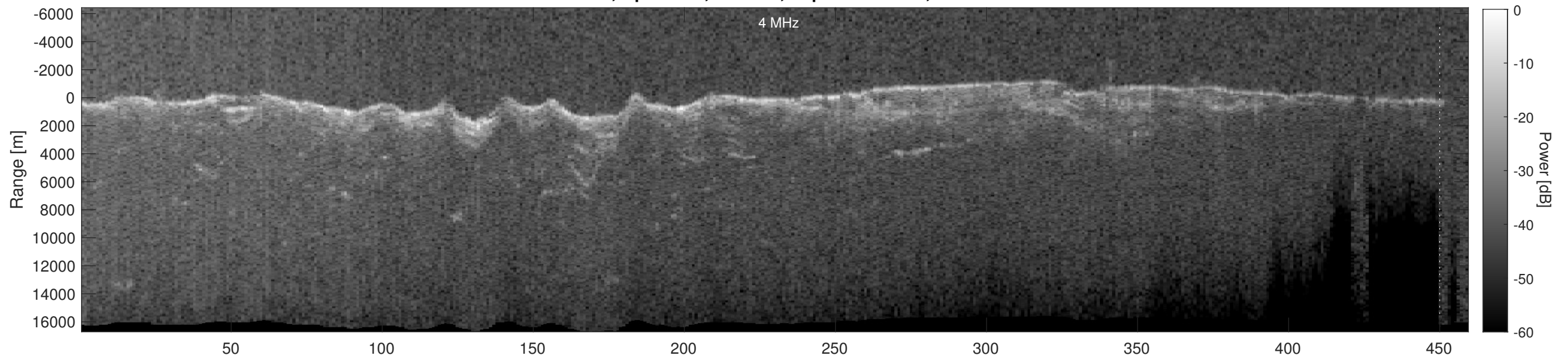
Orbit 4457, Depth-Corrected Cluttergram
