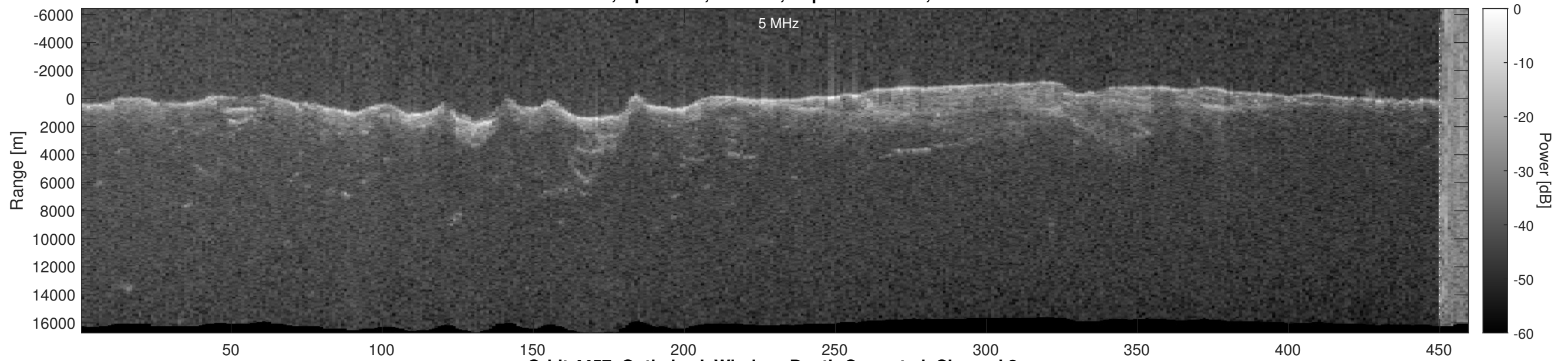
Orbit 4457, Optimized, Window, Depth-Corrected, Channel 2
