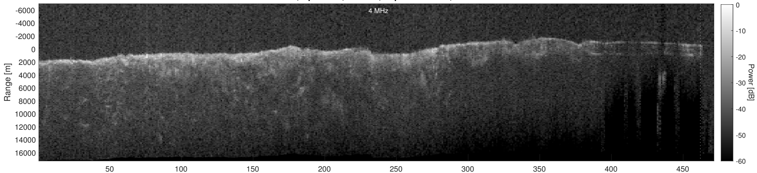
Orbit 4465, Depth-Corrected Cluttergram
