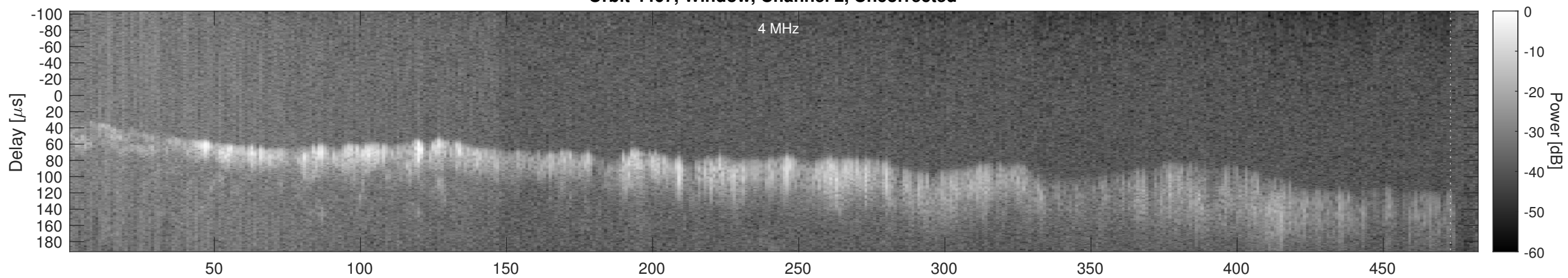
Orbit 4467, Window, Channel 2, Chapman
