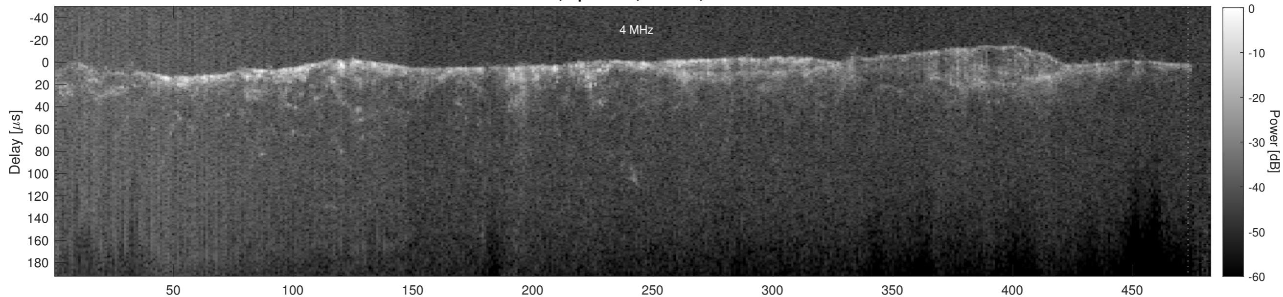
Orbit 4467, Cluttergram
