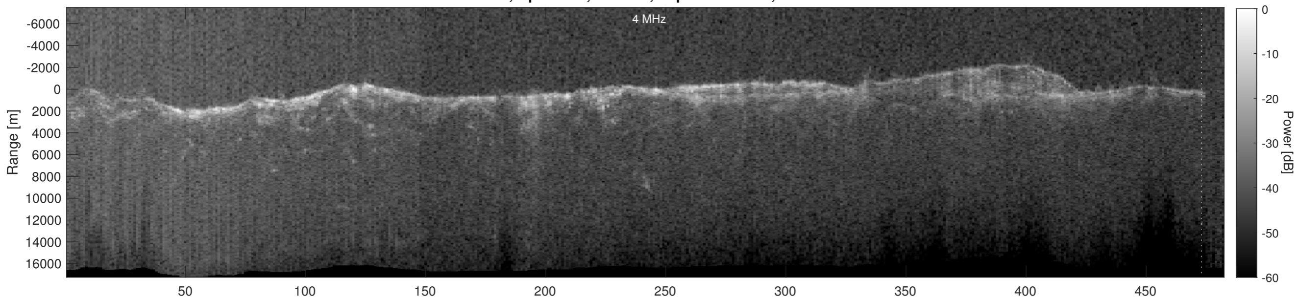
Orbit 4467, Depth-Corrected Cluttergram
