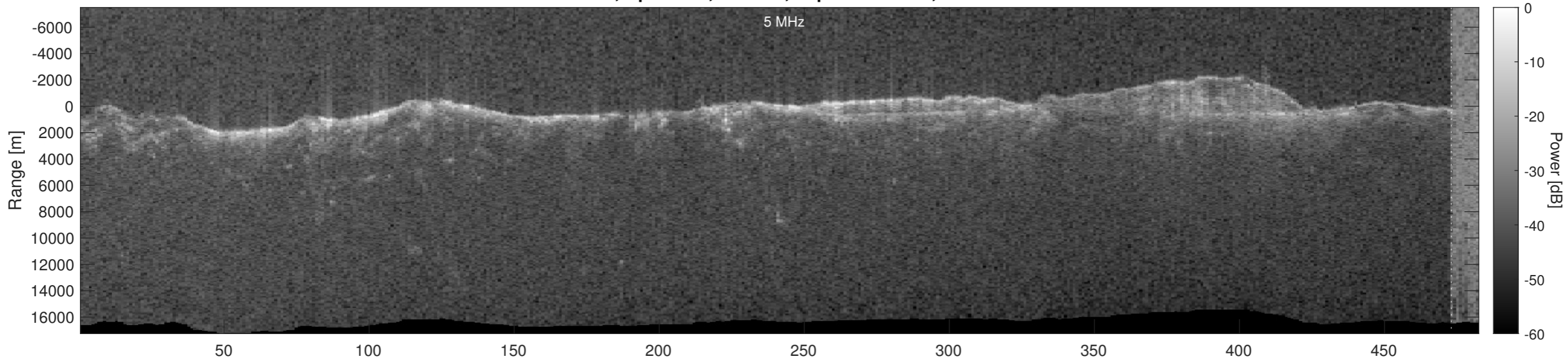
Orbit 4467, Optimized, Window, Depth-Corrected, Channel 2
