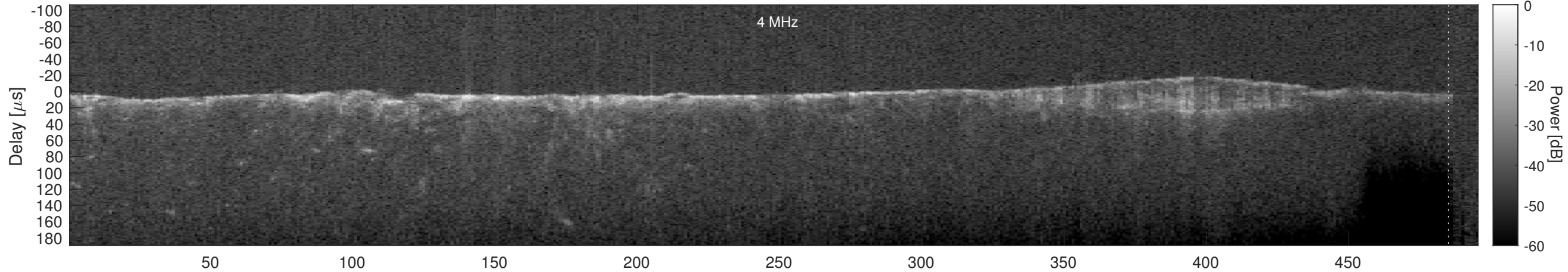
Orbit 4474, Cluttergram
