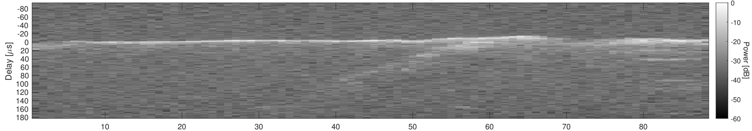
Orbit 4475, Window, Channel 2, Optimized
