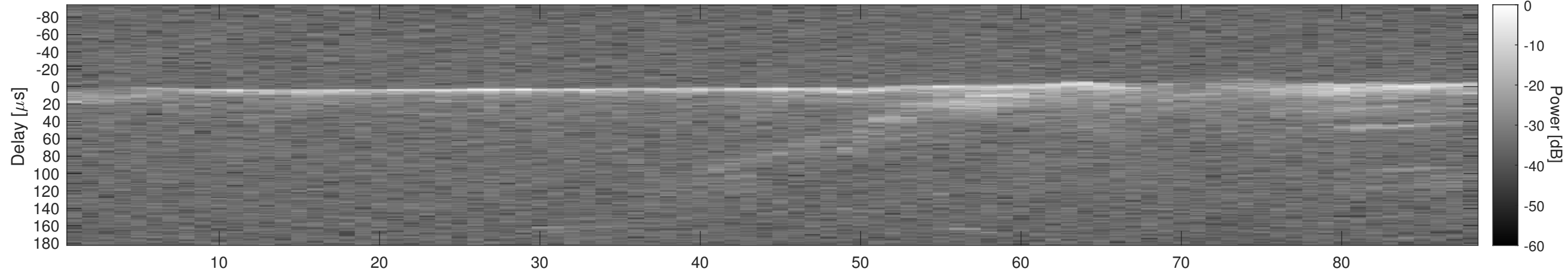
Orbit 4475, Cluttergram
