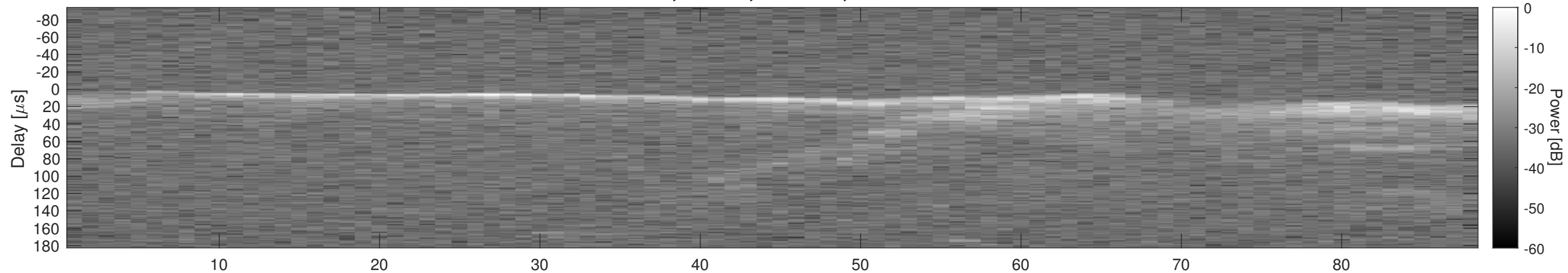
Orbit 4475, Window, Channel 2, Chapman
