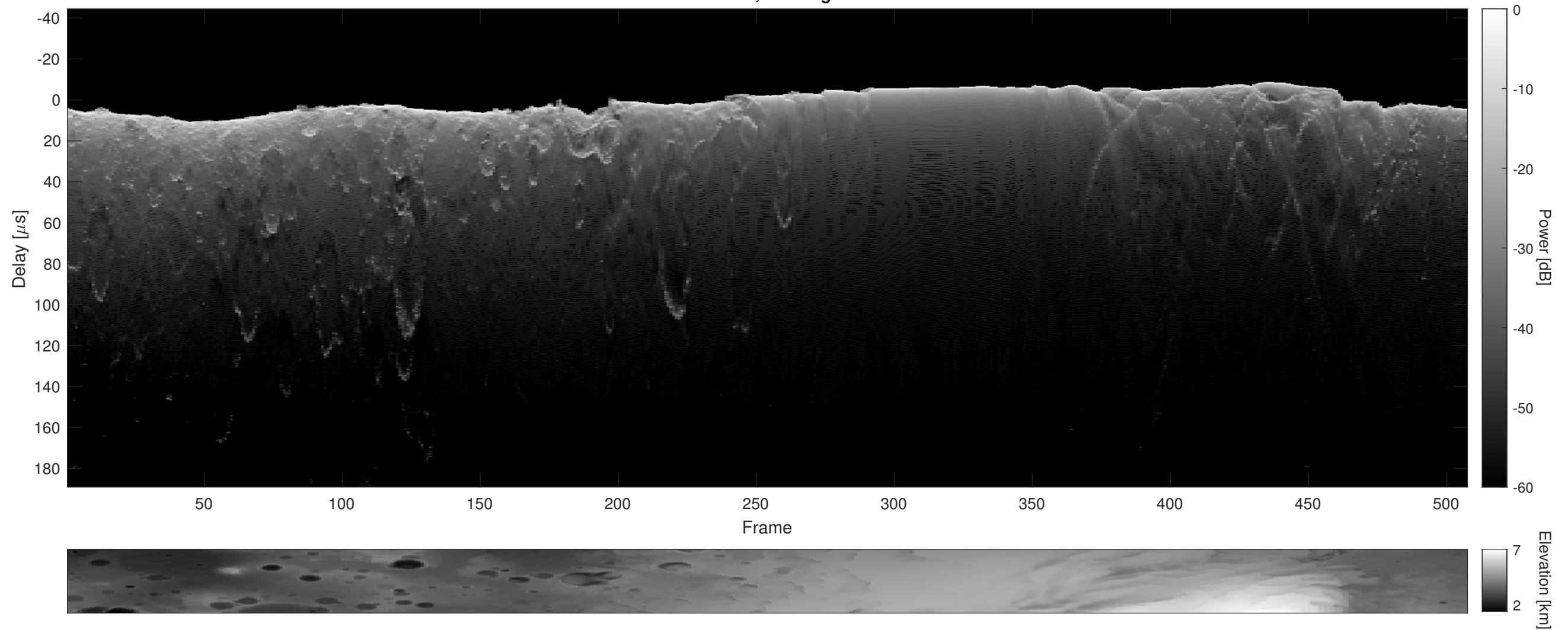
Orbit 4482, Cluttergram
