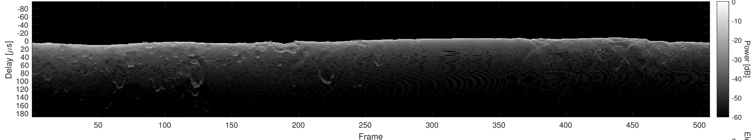
Orbit 4482, Cluttergram
