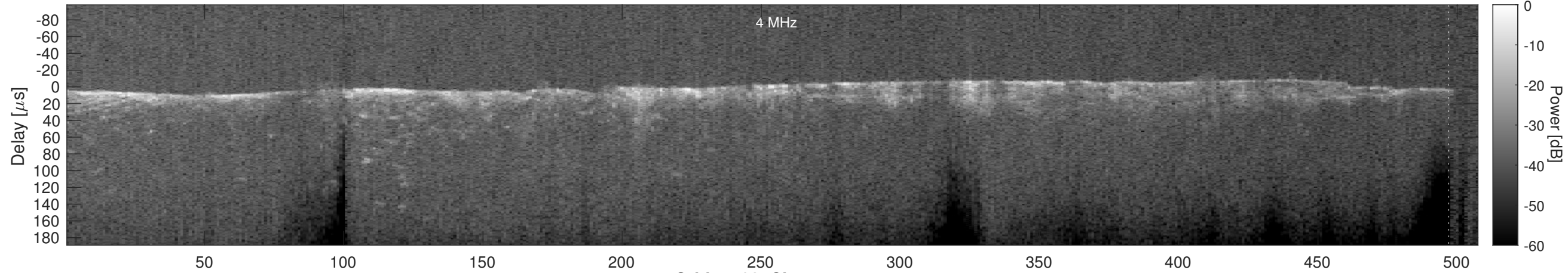
Orbit 4482, Cluttergram
