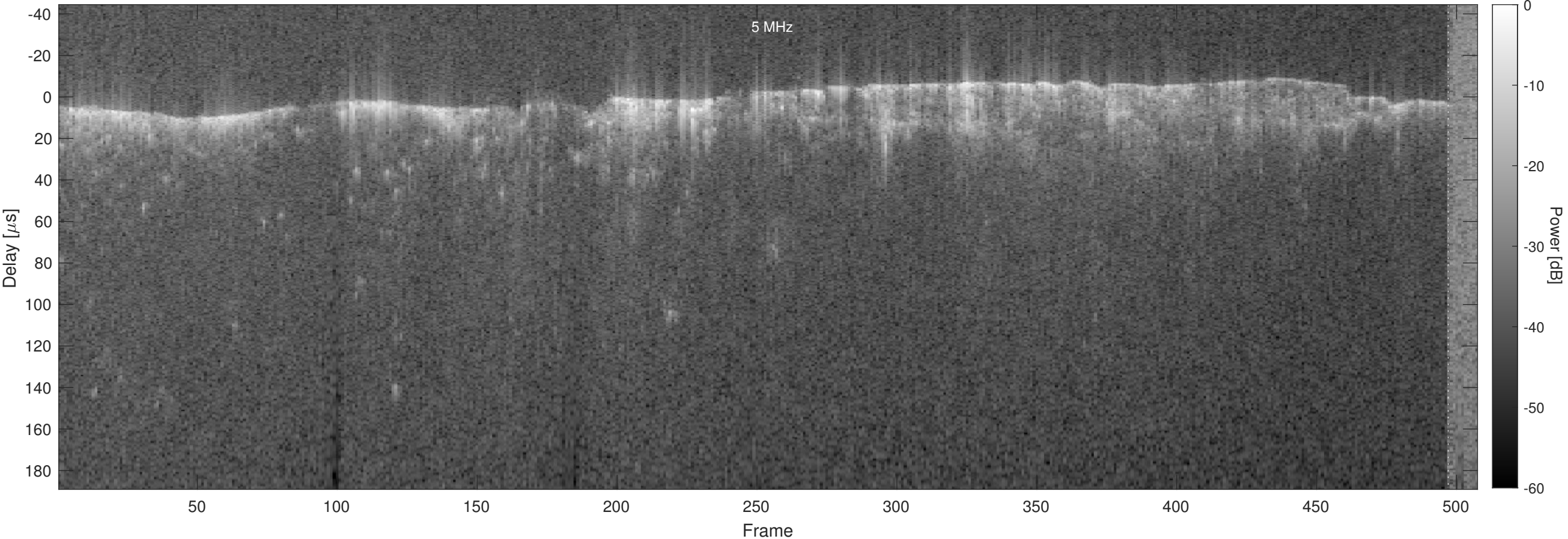
Orbit 4482, Optimized, No Window, Channel 2
