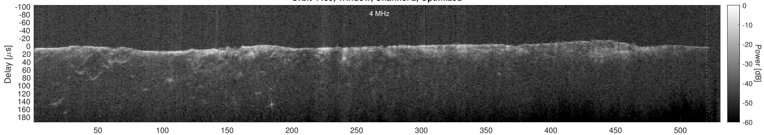
Orbit 4489, Cluttergram
