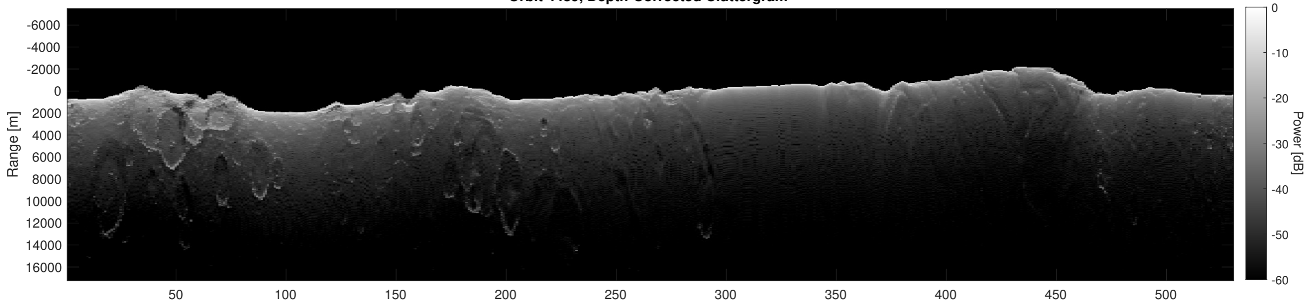
Orbit 4489, Depth-Corrected Cluttergram
