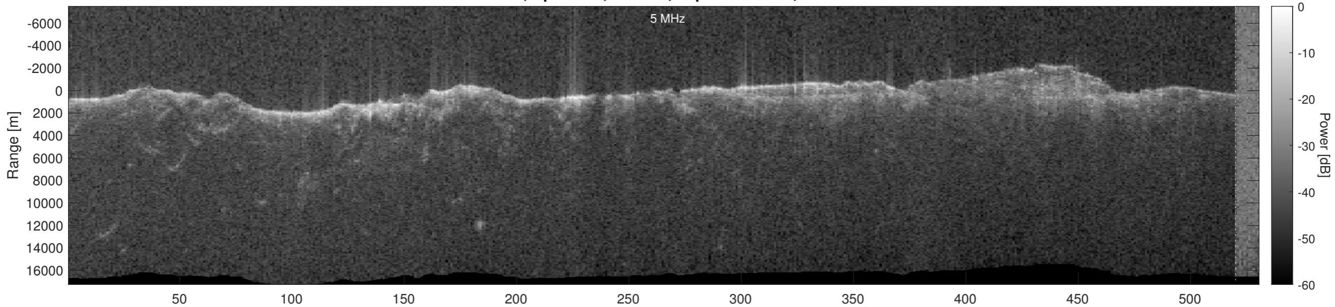
Orbit 4489, Optimized, Window, Depth-Corrected, Channel 2
