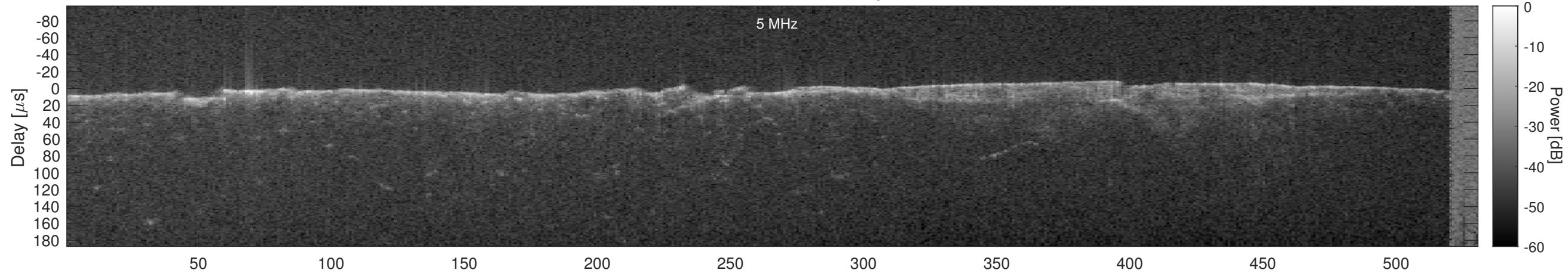
Orbit 4490, Cluttergram
