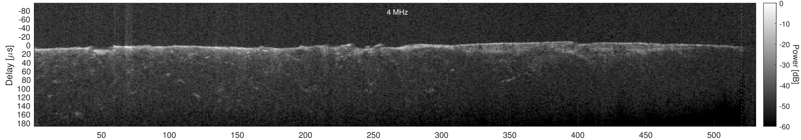
Orbit 4490, Cluttergram
