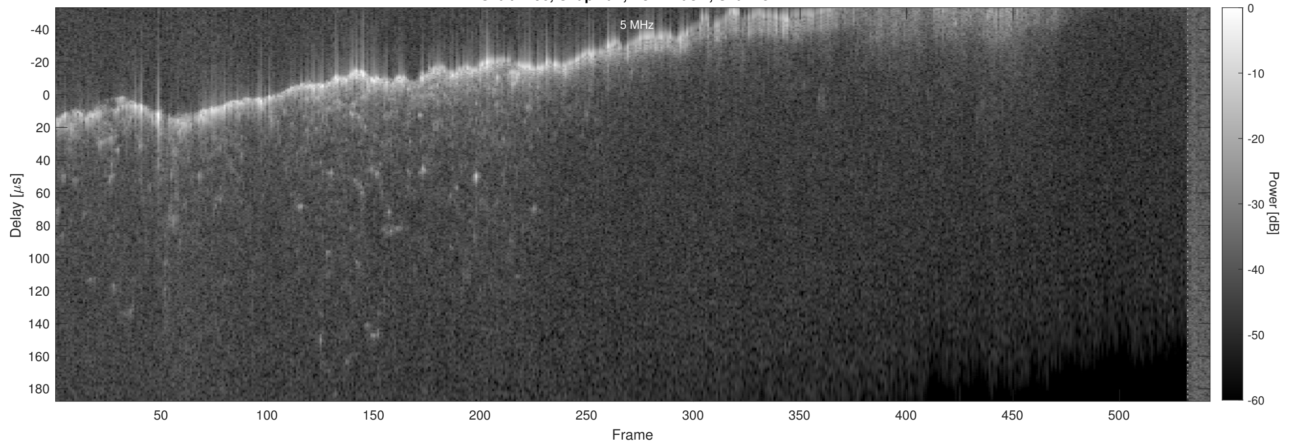
Orbit 4496, Chapman, No Window, Channel 2
