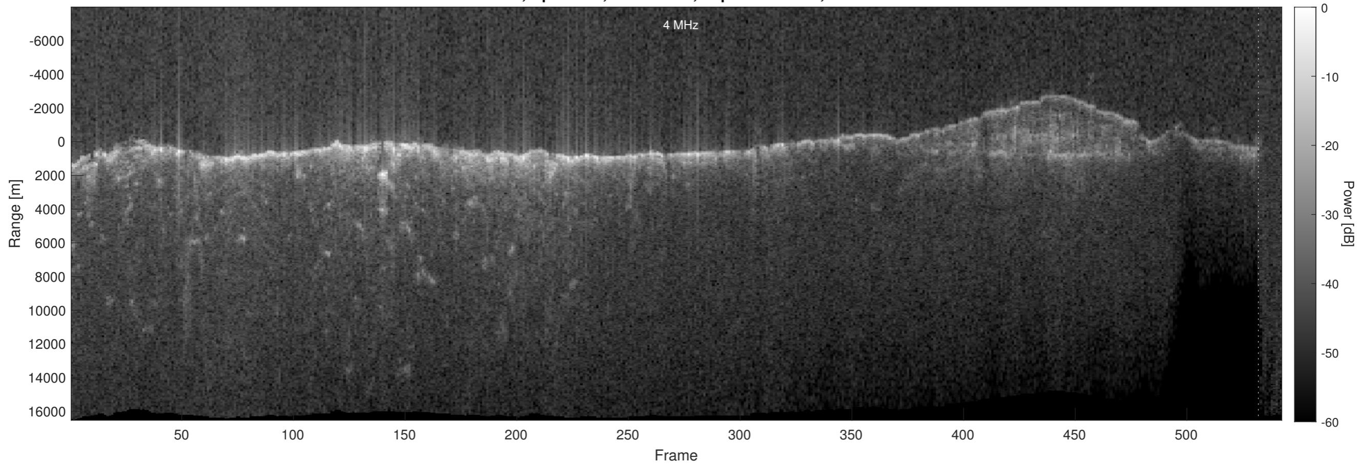
Orbit 4496, Optimized, No Window, Depth-Corrected, Channel 2
