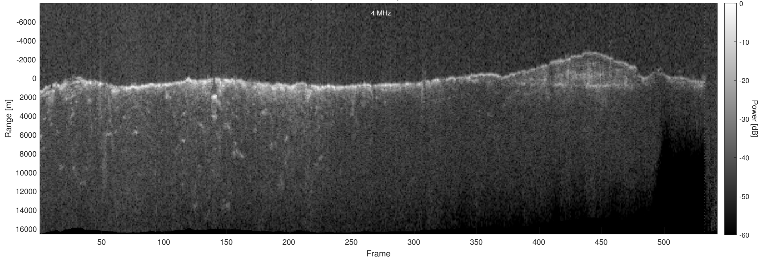
Orbit 4496, Optimized, Window, Depth-Corrected, Channel 2
