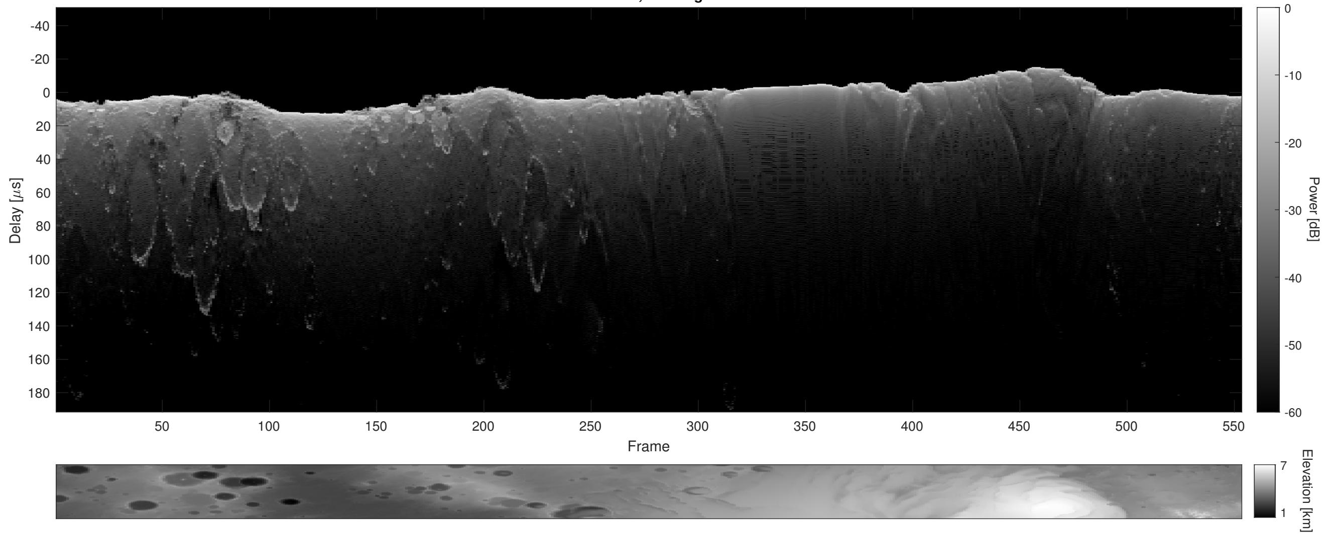
Orbit 4500, Cluttergram
