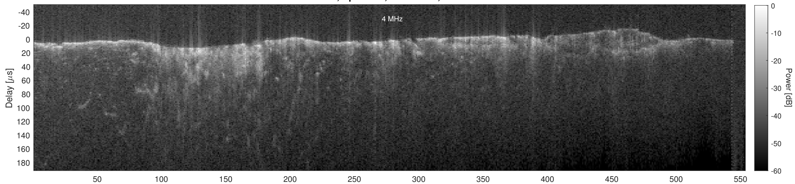
Orbit 4500, Cluttergram
