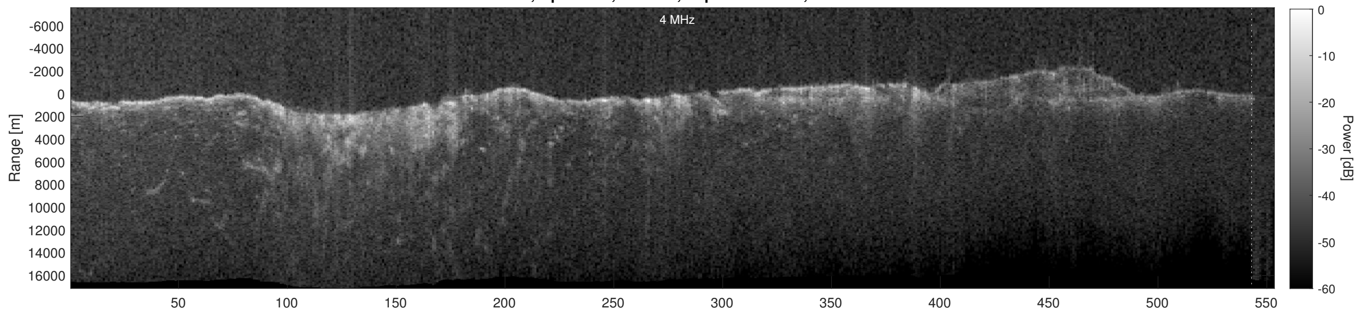
Orbit 4500, Depth-Corrected Cluttergram
