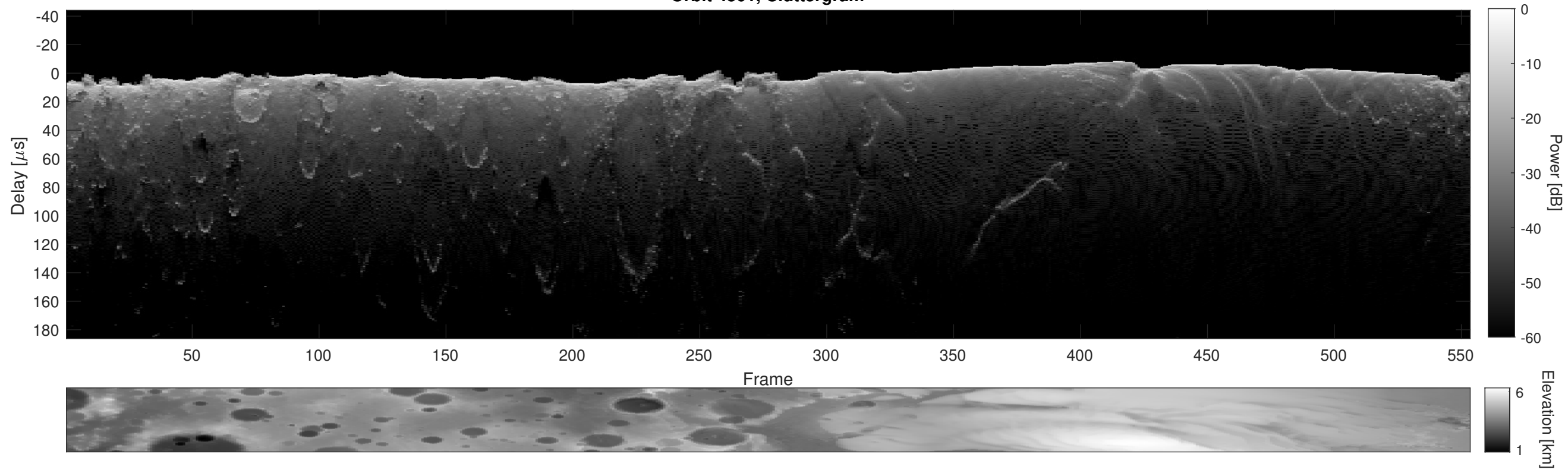
Orbit 4501, Cluttergram
